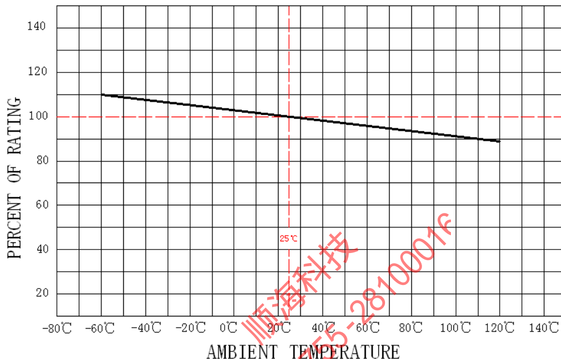
Temperature-Current curve:
